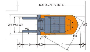
RASA Aisle width with load a. Clearance b. Load Length
